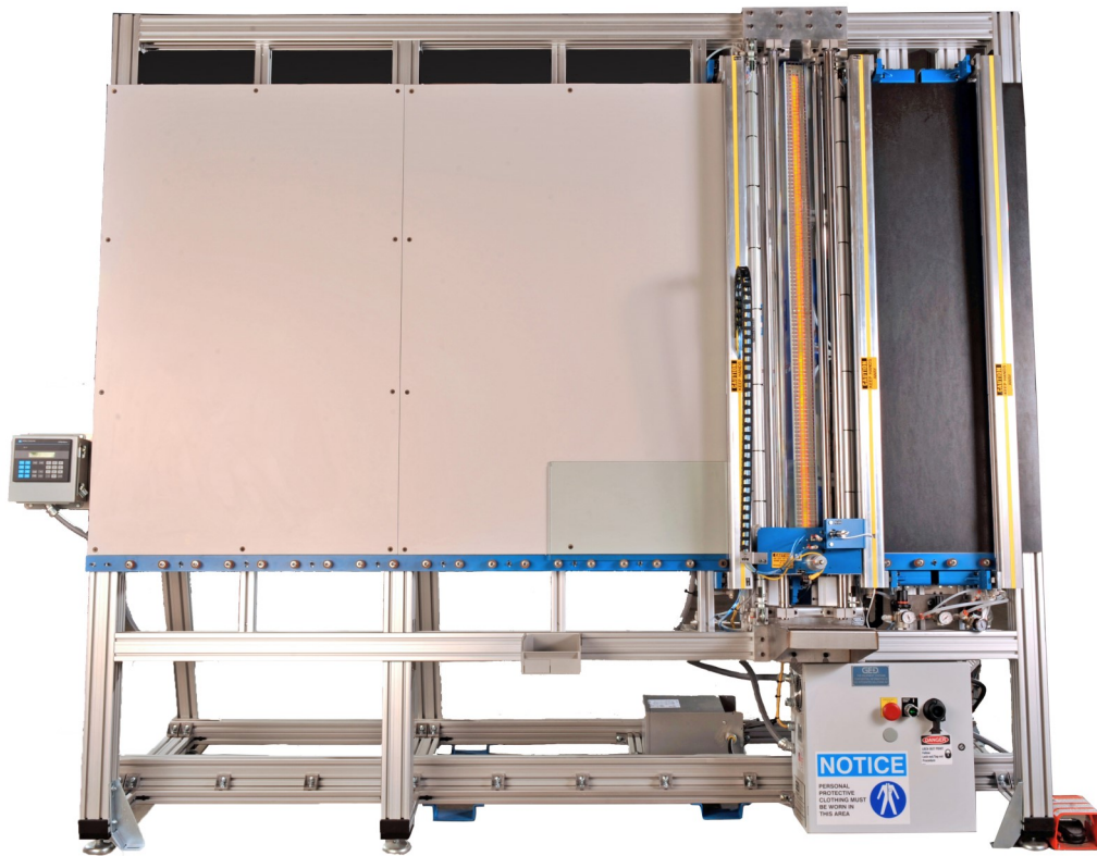
Laminated Glass Cutting with Multiple Functionality
